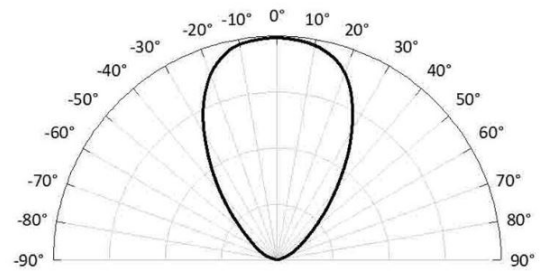
Radiation Pattern
