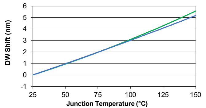
Dominant Wavelength Shift Vs Junction Temperature
