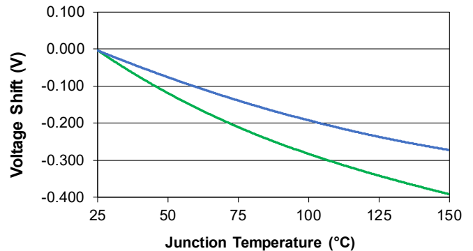
Voltage Shift Vs Junction Temperature
