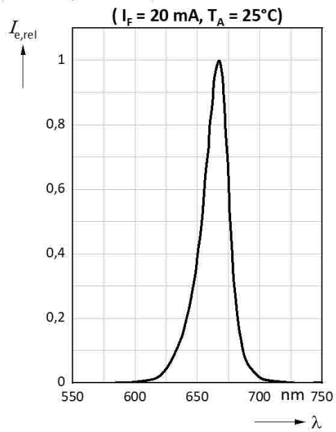
Spectrum (Relative Spectral Emission vs. Wavelength)
