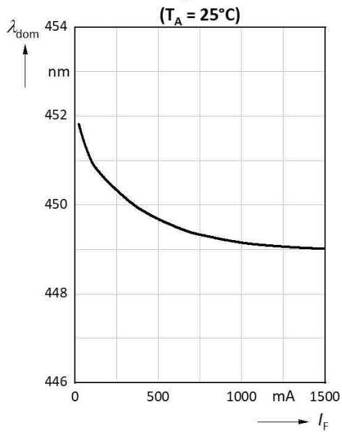
Dominant Wavelength vs. Forward Current
