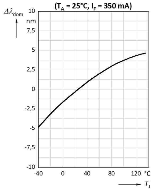
Dominant Wavelength Shift vs. Junction Temperature
